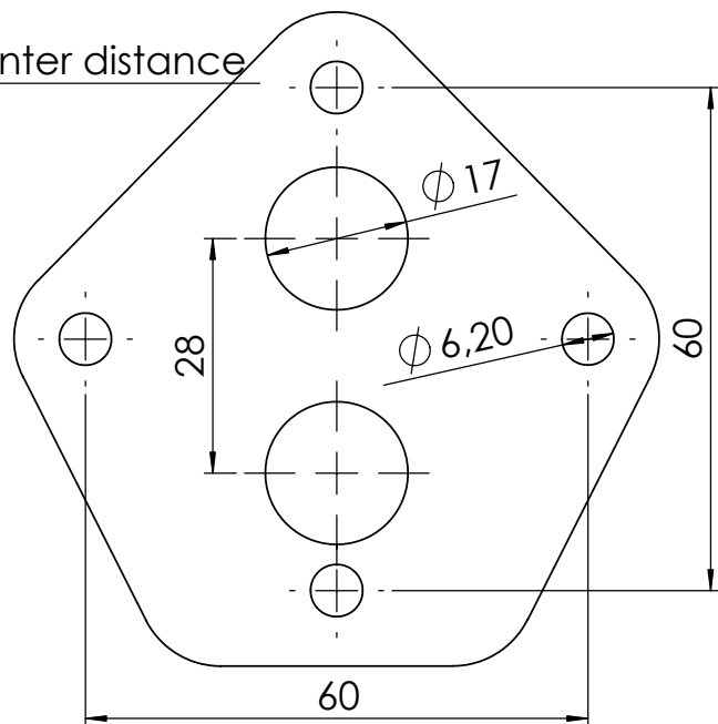
Drilling Jig Scale 1:1
